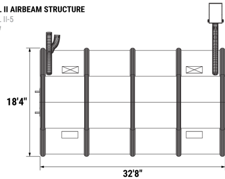
SENTINEL II AIRBEAM STRUCTURE SENTINEL II-5 RIGHT SIDE VIEW
