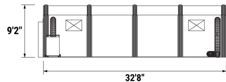
SENTINEL II AIRBEAM STRUCTURE SENTINEL II-5 RIGHT SIDE VIEW
