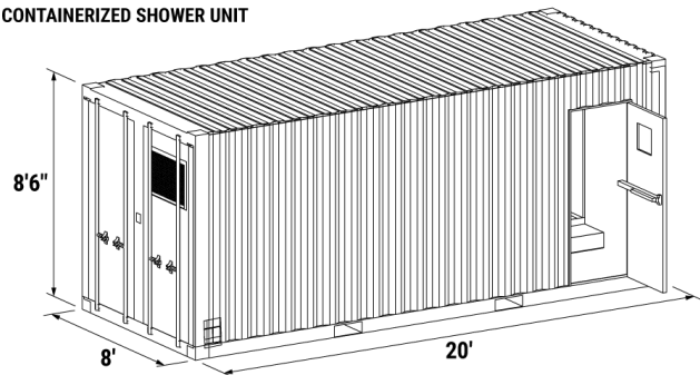
CONTAINERIZED SHOWER UNIT
