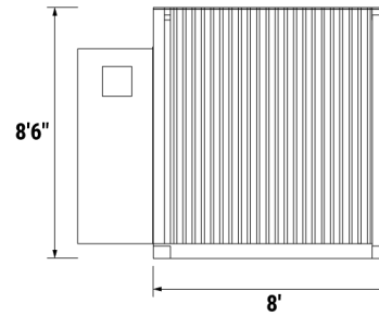
CONTAINERIZED SHOWER UNIT RIGHT SIDE VIEW
