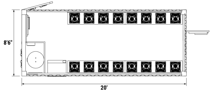
CONTAINERIZED SINK UNIT TOP VIEW
