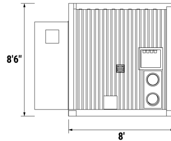
BICON LAUNDRY UNIT RIGHT SIDE VIEW
